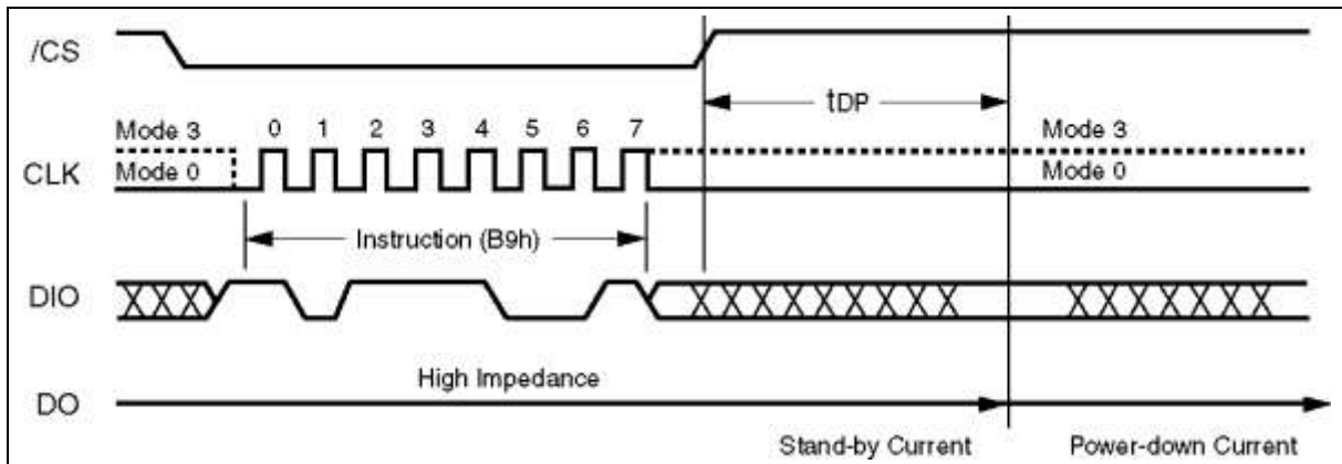
Figure 18. Deep Power-down Instruction Sequence Diagram
