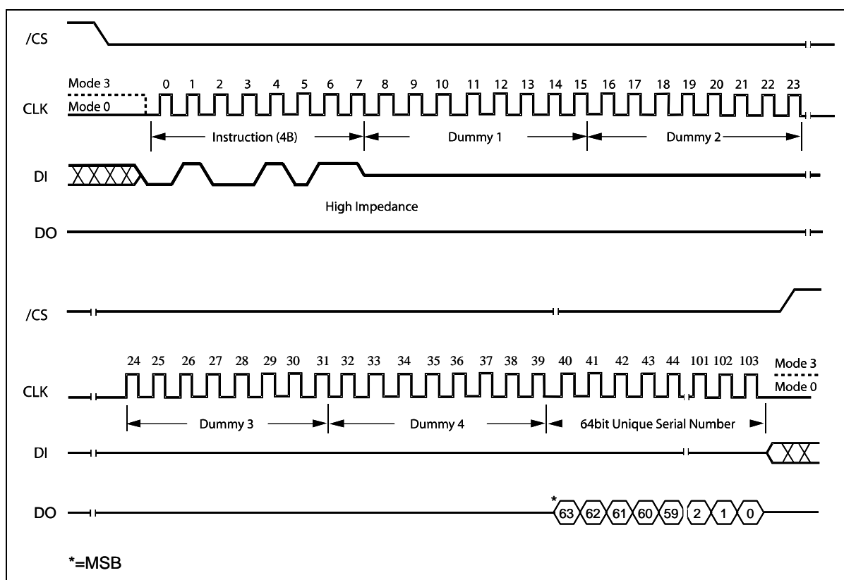
Figure 23. Read Unique ID Number Instruction Sequence
