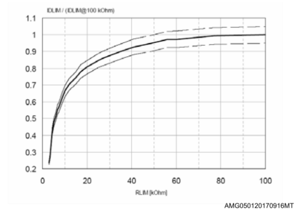
Figure 16: Current limit vs R_{LIM}
