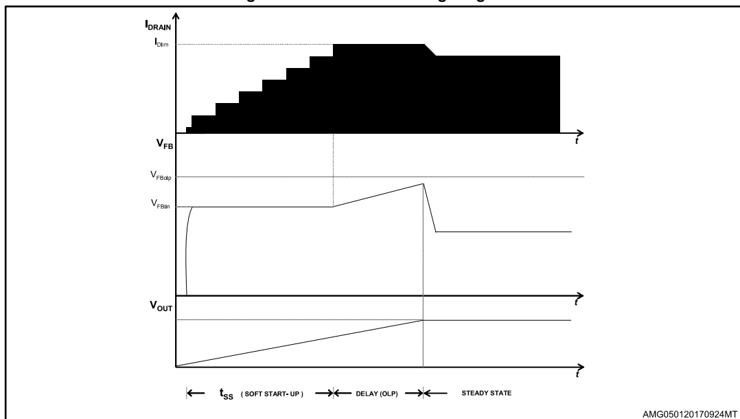
Figure 24: Soft-start: timing diagram
