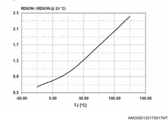
Figure 17: Power MOSFET on-resistance vs T_J
