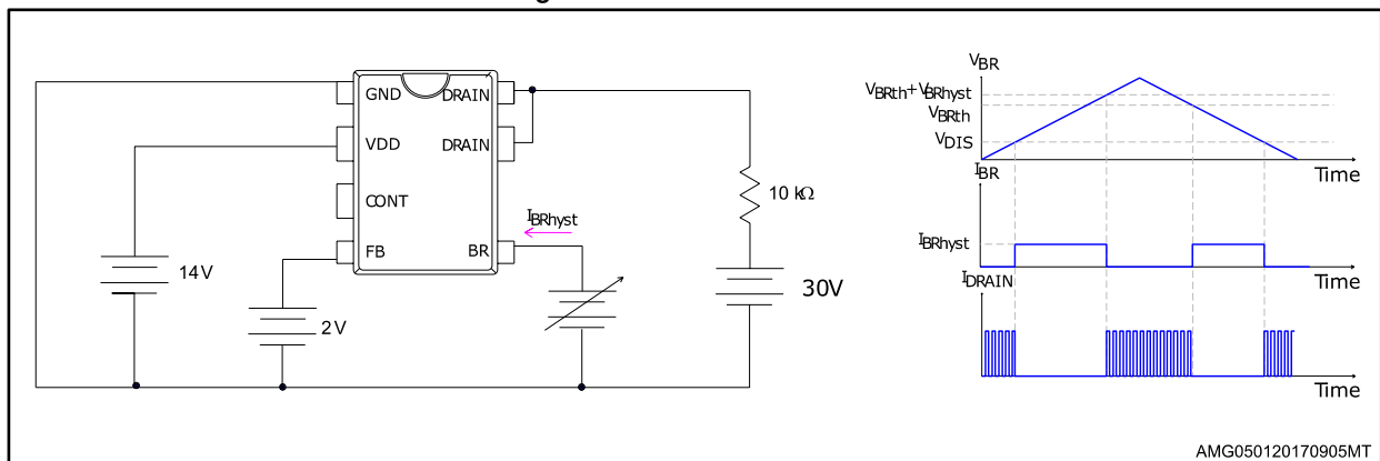
Figure 5: Brown out threshold test circuit
