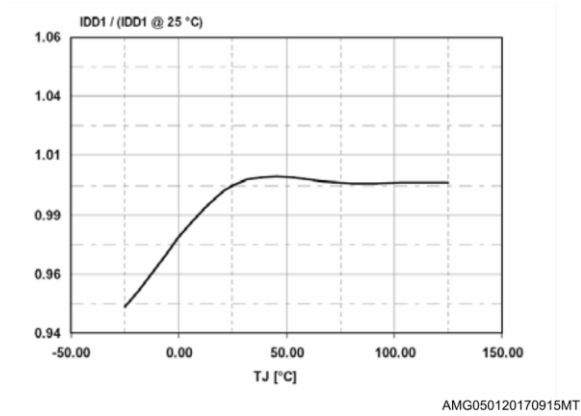
Figure 15: Operating supply current (switching) vs T_J
