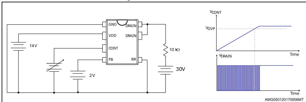
Figure 6: OVP threshold test circuit
