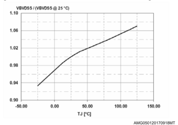
Figure 18: Power MOSFET break down voltage vs T_J
