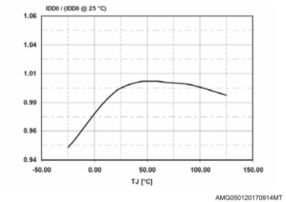
Figure 14: Operating supply current (no switching) vs T_J
