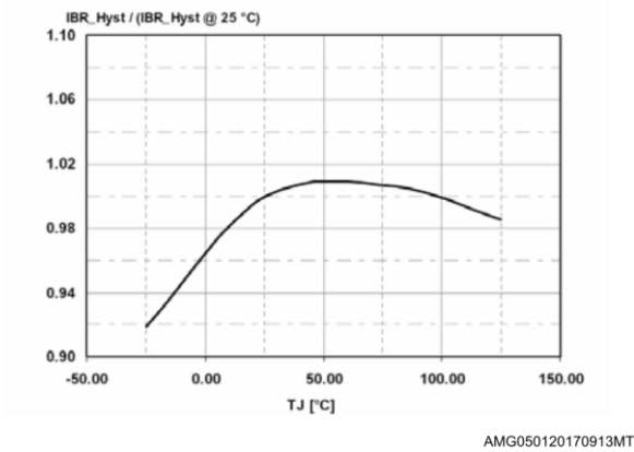
Figure 13: Brown out hysteresis current vs T_J
