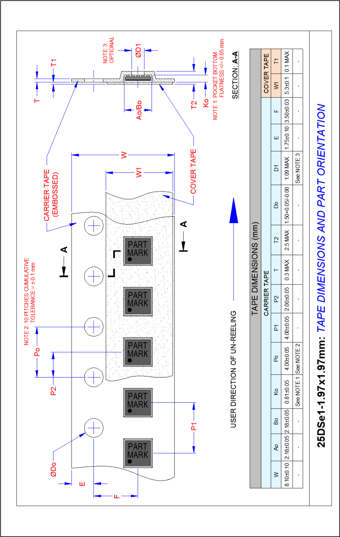
Figure 9.2 25WLCSP, 1.97x1.97 Tape and Reel
