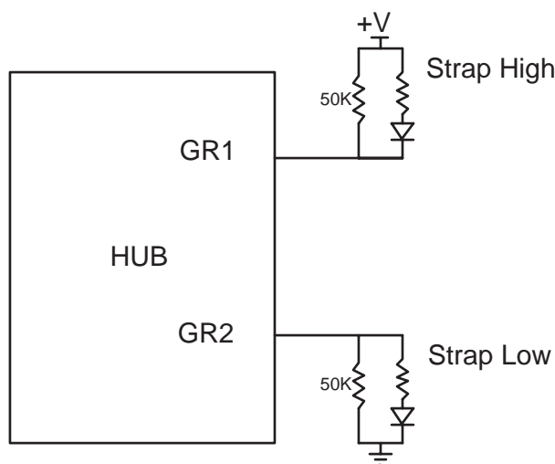
Figure 5.1 LED Strapping Option
