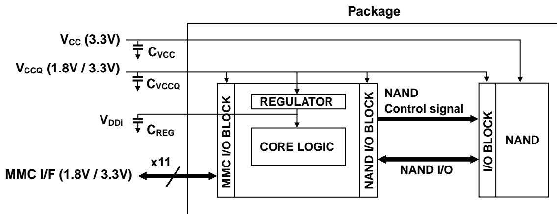
Figure 1 THGBMNG5D1LBAIT Block Diagram
