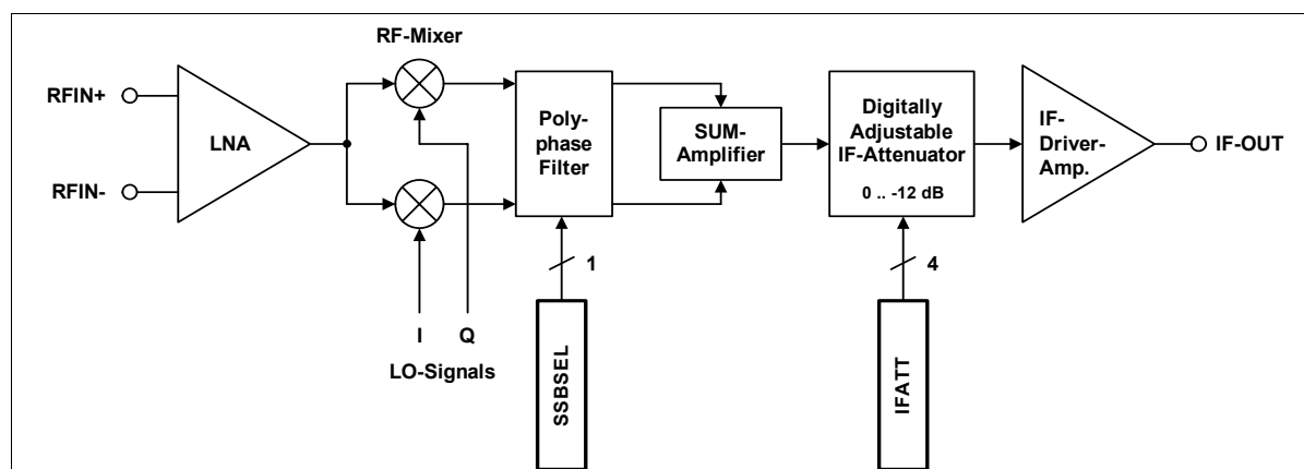
Figure 29 RF Path
