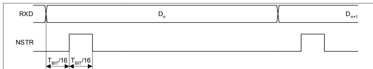
Figure 63 Transparent Mode
