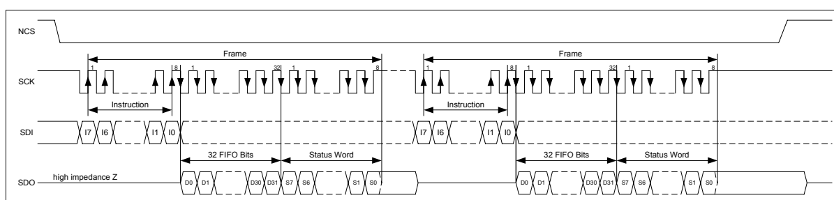
Figure 68 Read FIFO
