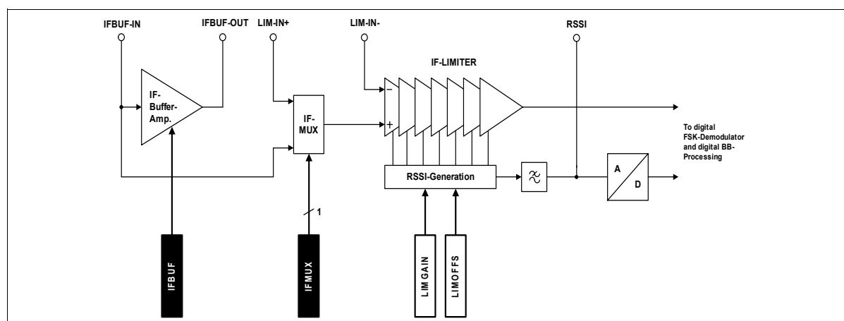
Figure 30 IF Path
