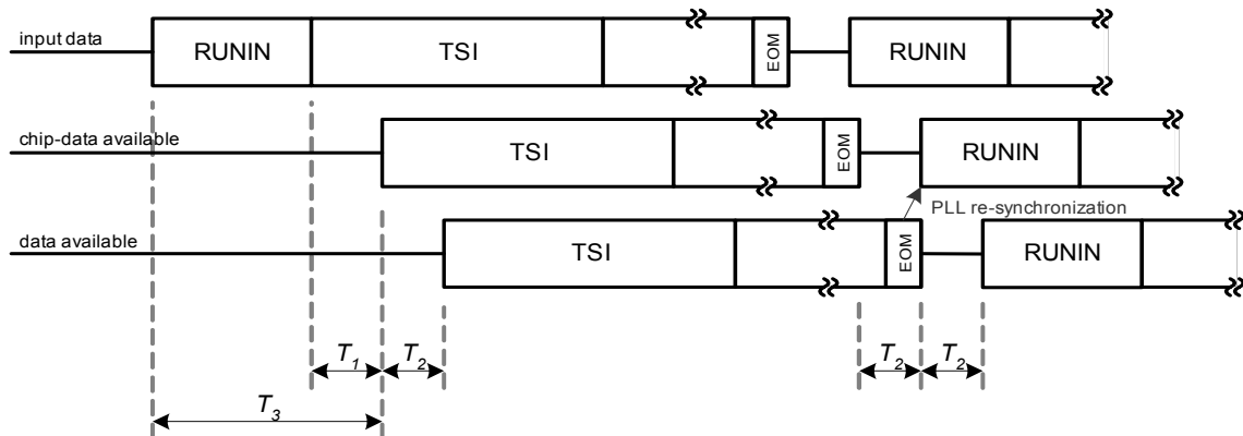
Figure 39 Data Latency
