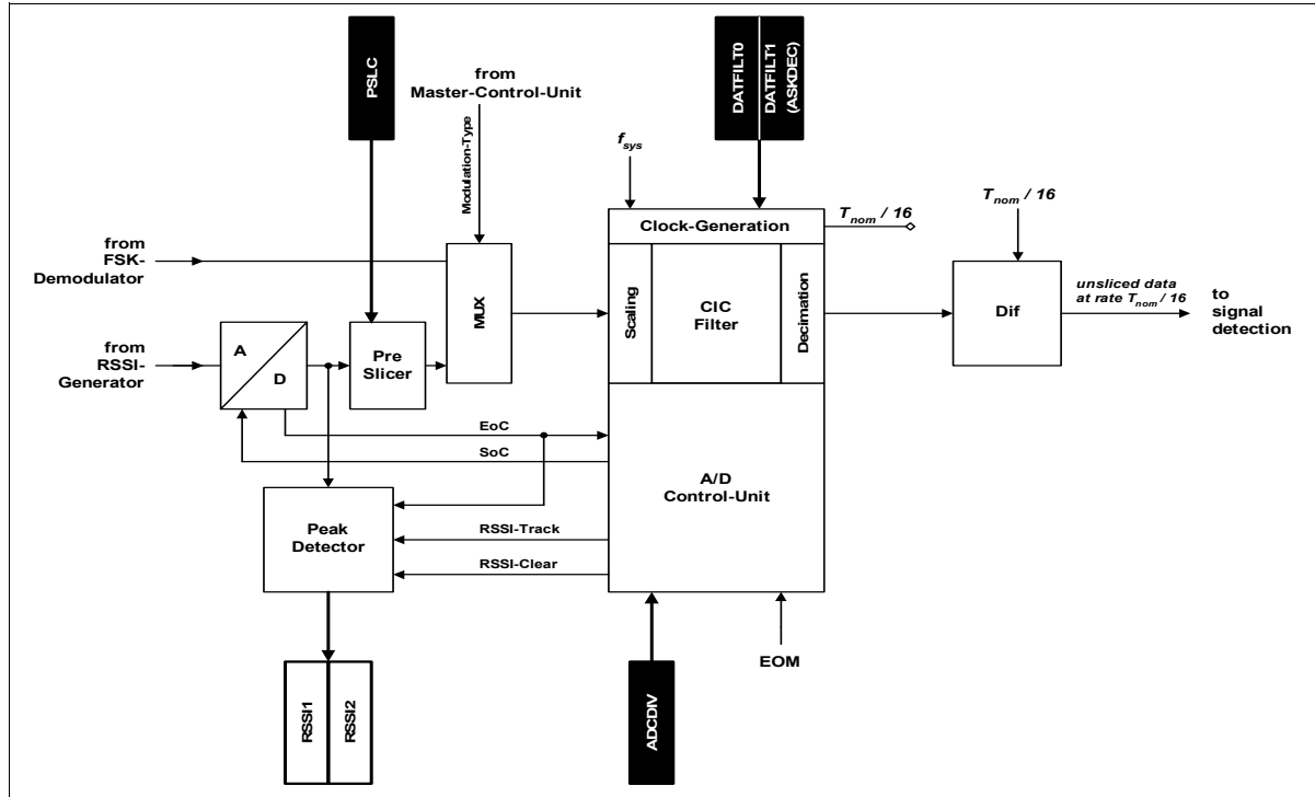
Figure 40 AD-Control and Matched-Filter
