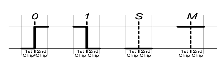
Figure 37 Manchester Code
