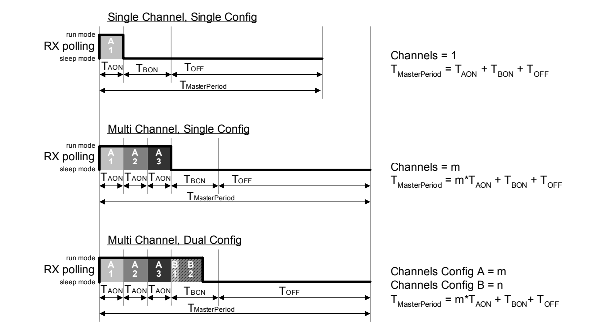
Figure 26 Mixed Mode
