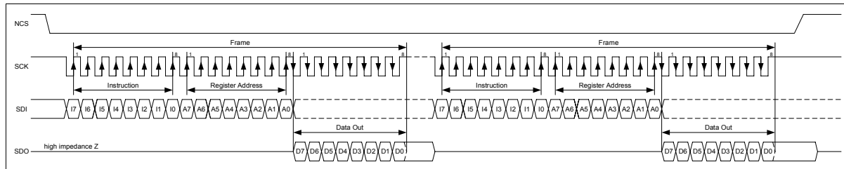
Figure 66 Read Register
