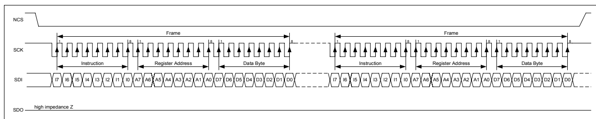
Figure 67 Write Register
