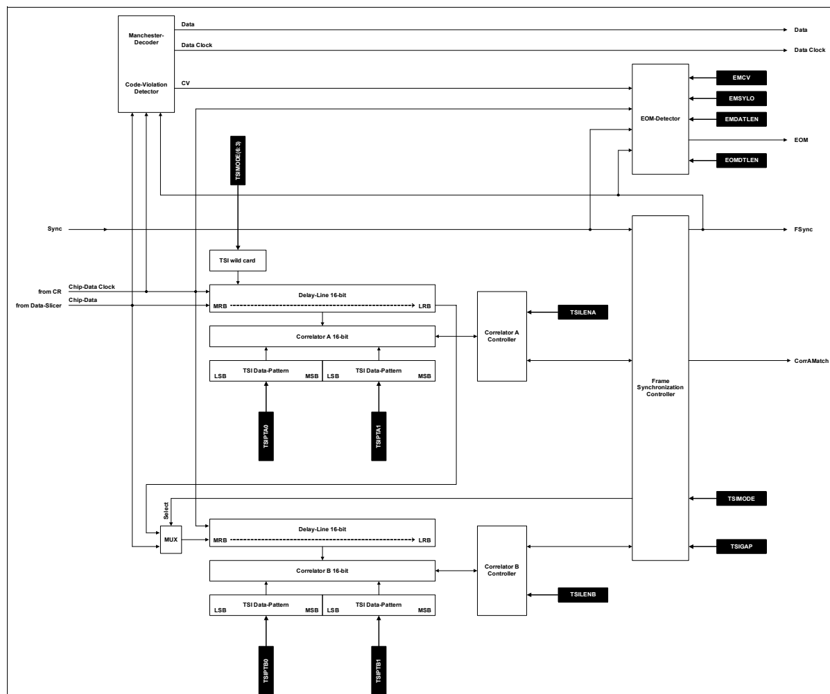
Figure 48 Frame Synchronisation Unit
