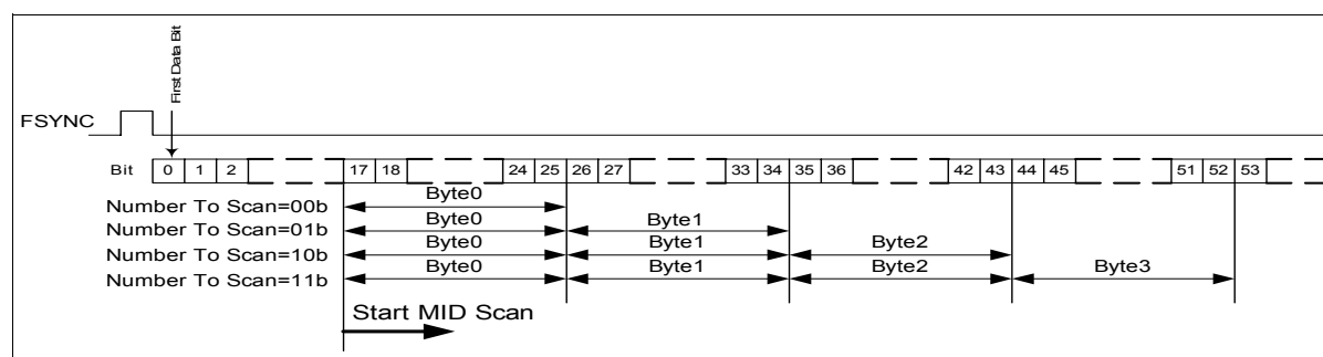
Figure 59 ID Scanning
