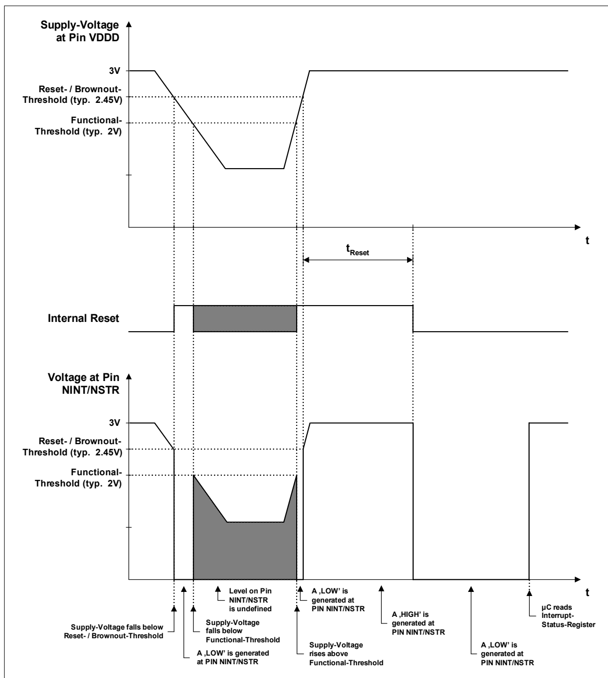
Figure 13 Reset Behavior
