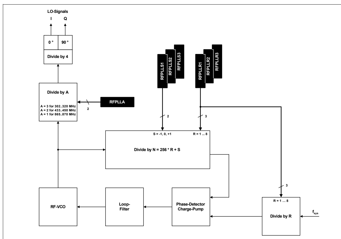
Figure 16 RF PLL
