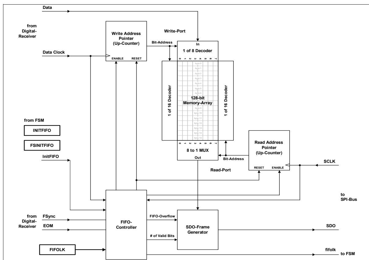
Figure 60 Data FIFO
