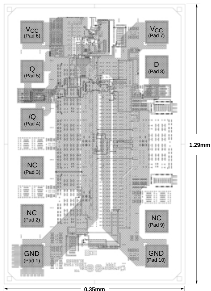
Figure 1. Chip Topography
