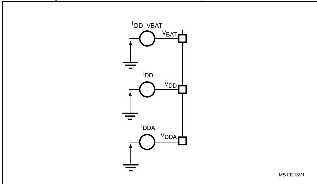
Figure 12. Scheme of the current-consumption measurement
