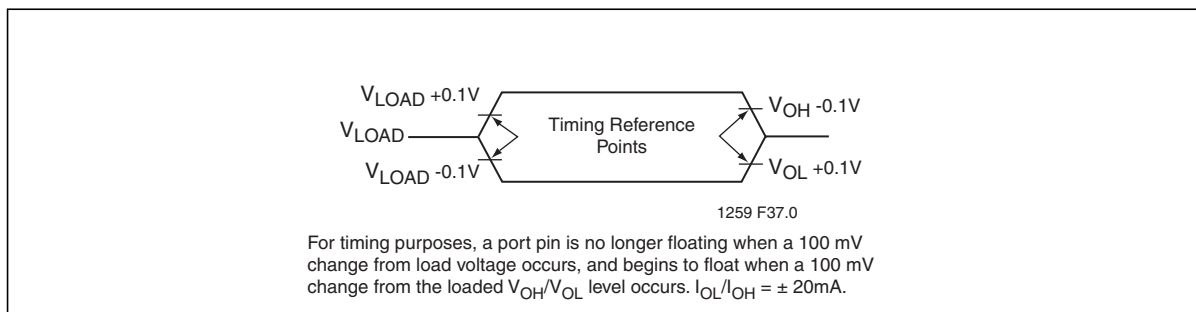
Figure 22: Float Waveform
