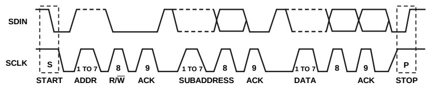
Figure 24. 2-Wire I 2 C Generalized Clocking Diagram
