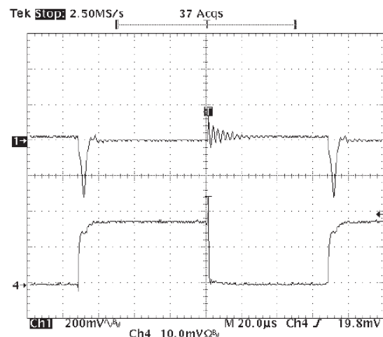
Fig. 17: Load Step Response 0mA to 800mA V_{IN}=3.3V , V_{OUT}=1.8V , C_{IN}=10\mu F , C_{OUT}=2.2\mu F , OSCON Signal 1= V_{OUT} , Signal 4= I_{LOAD}
