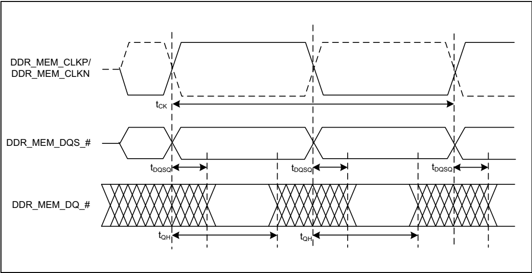
Figure 10. DDR2/LPDDR read cycle waveform
