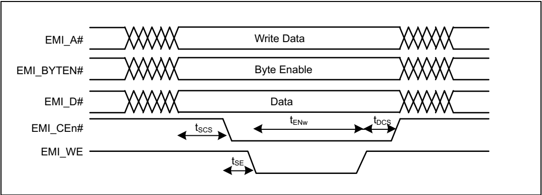
Figure 16. EMI write cycle waveform without acknowledgement on EMI_WAIT
