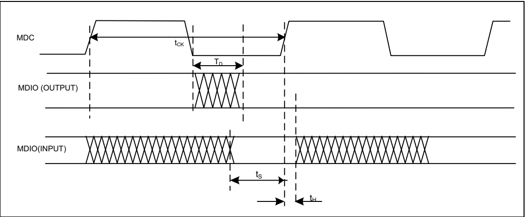
Figure 19. MDC waveform
