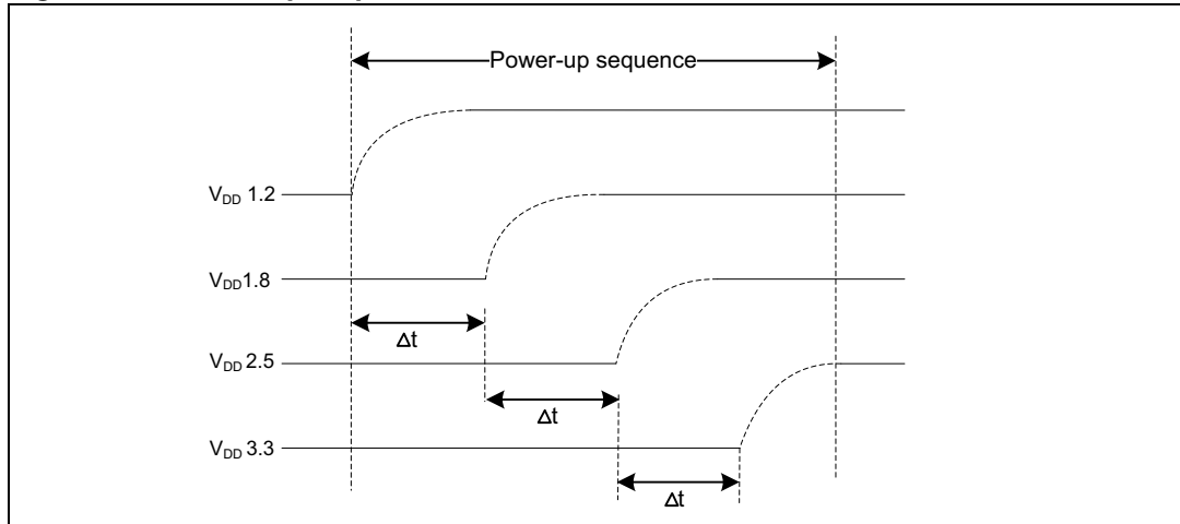
Figure 6. Power-up sequence
