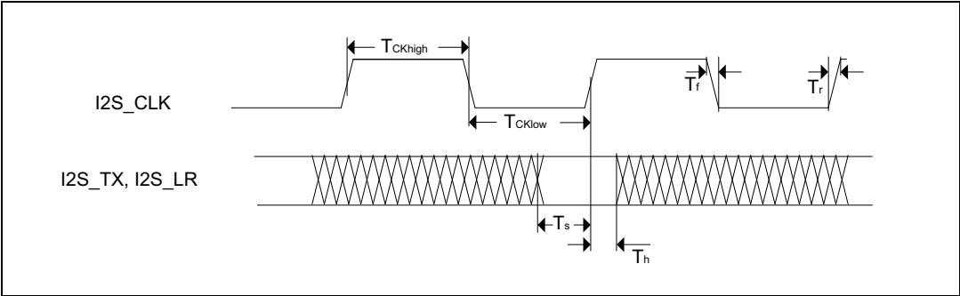
Figure 27. I2S waveform
