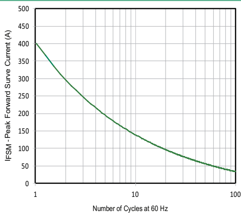
Figure 7 - Maximum Non-Repetitive Peak Forward Surge Current Uni-Directional Only
