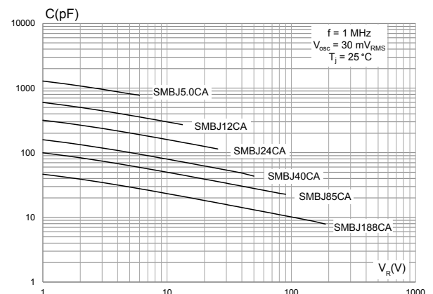
Figure 8. Junction capacitance versus applied voltage (bidirectional types)
