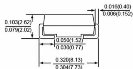
SMC/DO-214AB
