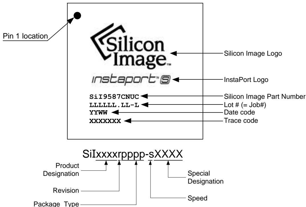
Figure 7.2. Marking Diagram
