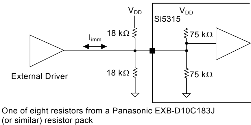
Figure 4. Three Level Input Pins
