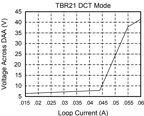
Figure 22. TBR21 Mode I/V Characteristics, DCV[1:0] = 11, MINI[1:0] = 00, ILIM = 1
