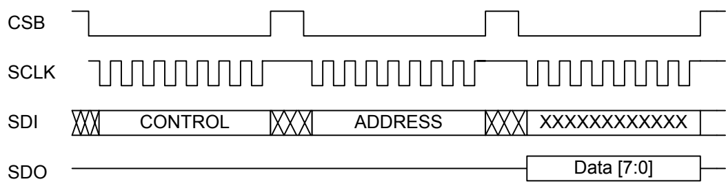
Figure 38. Read Operation via an 8-bit SPI Port
