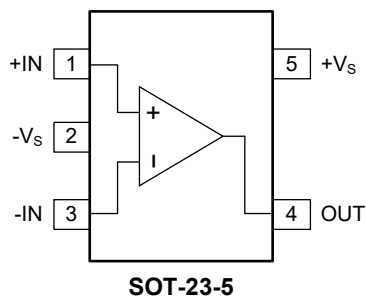
SGM8271BYN5G (TOP VIEW)
