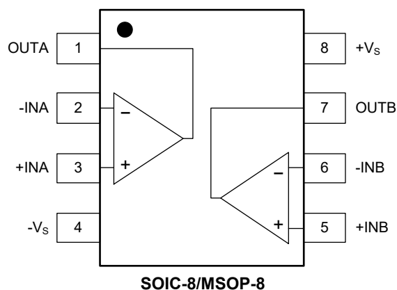
SGM8272 (TOP VIEW)
