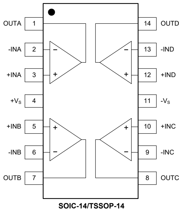
SGM8274 (TOP VIEW)
