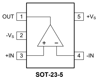
SGM8271AYN5G (TOP VIEW)
