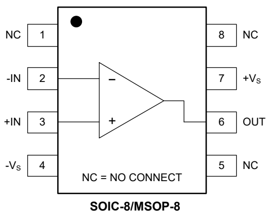
SGM8271 (TOP VIEW)
