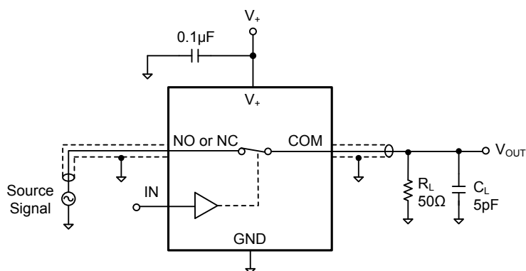
Test Circuit 8. -3dB Bandwidth
