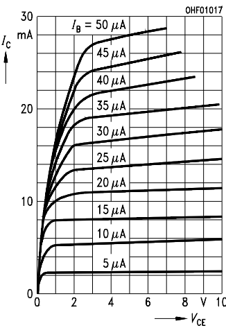
Collector Current Kollektorstrom I_C = f(V_{CE}), I_B = \text{Parameter}
