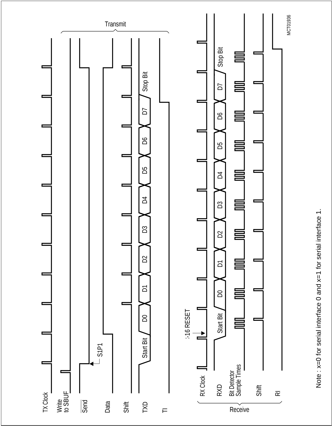
Figure 6-39 Timing Diagram - Serial Interfaces 0 and 1, Mode 1 / Mode B
