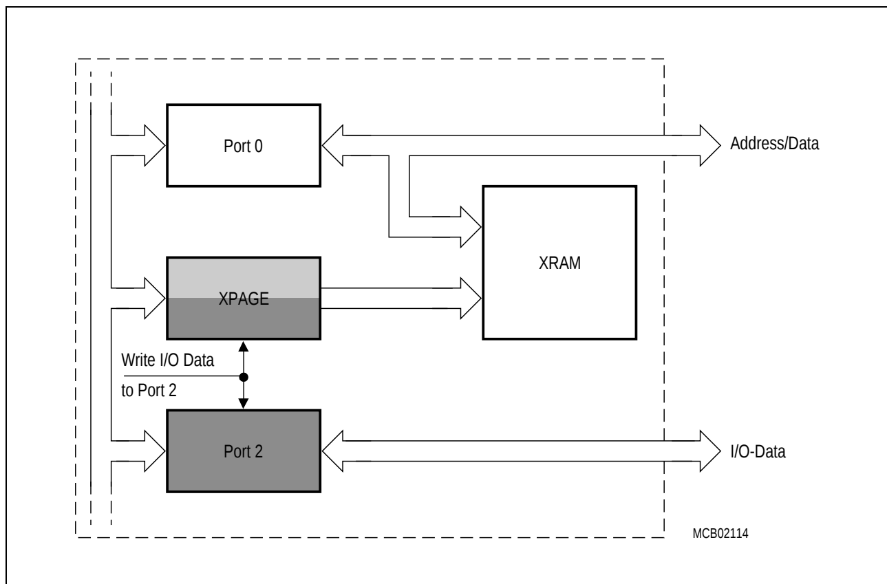
Figure 3-4 Usage of Port 2 as I/O Port
