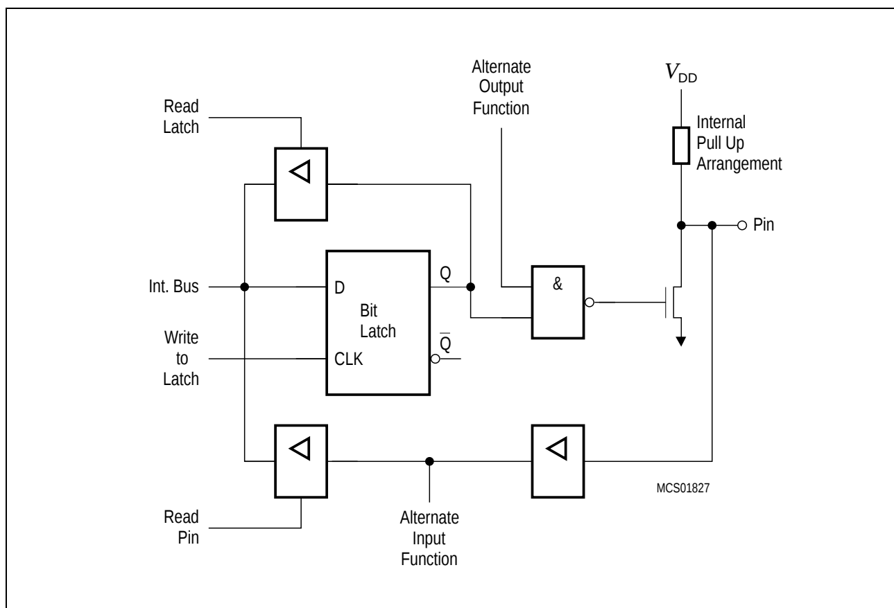
Figure 6-4 Ports 1, 3, 4, 5, and 6
