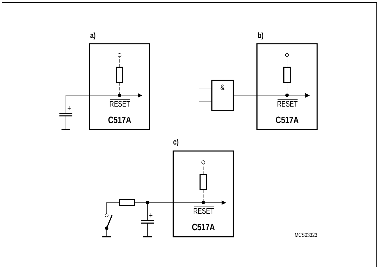
Figure 5-1 Reset Circuitries
