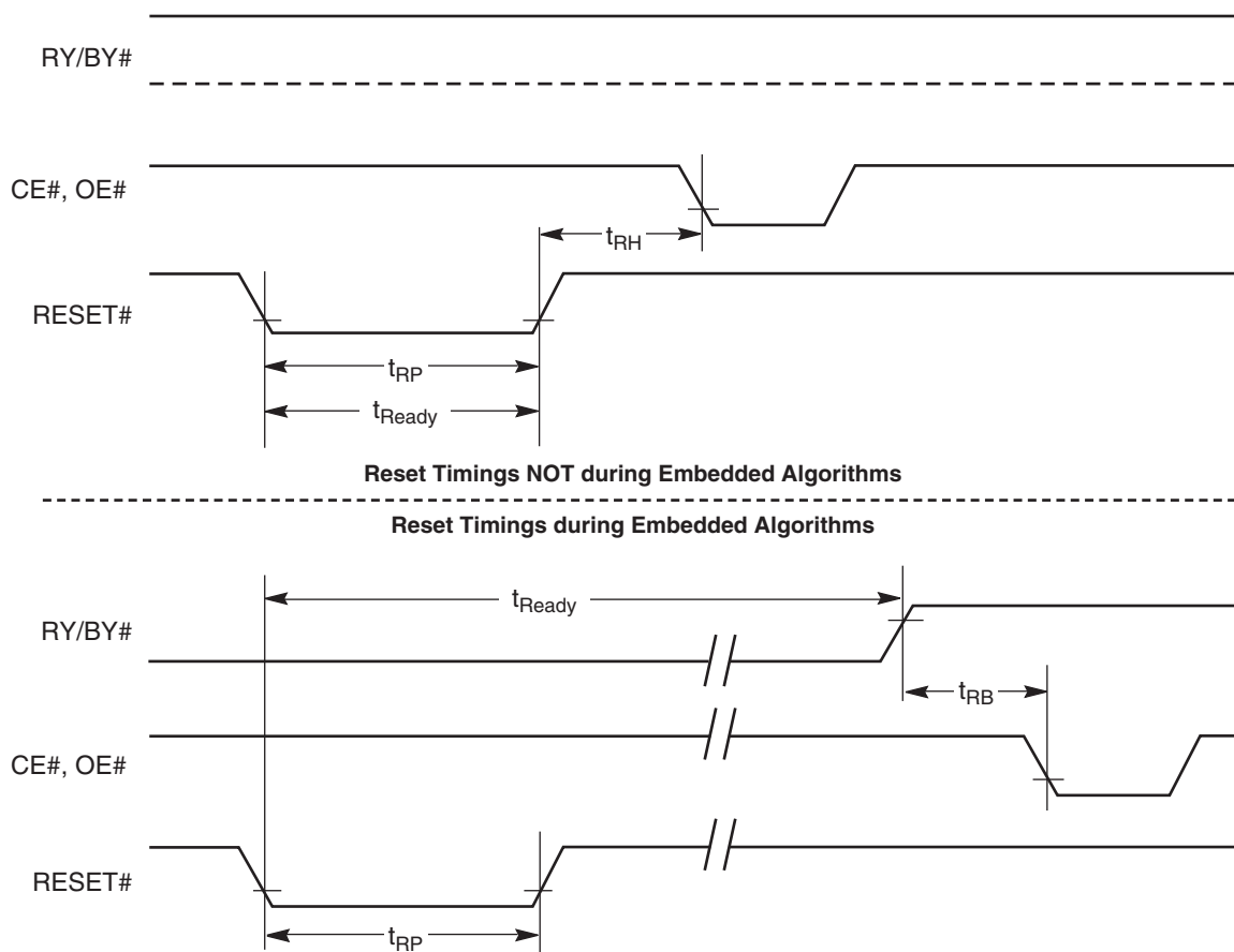
Figure 18. Reset Timings
