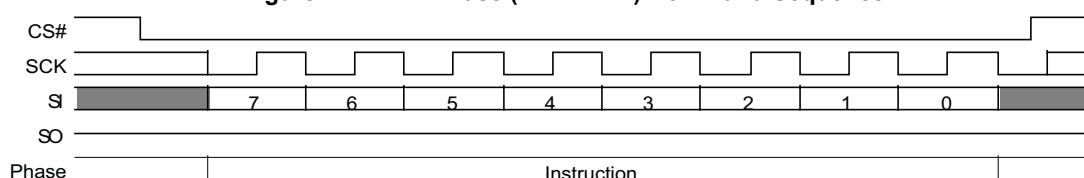
Figure 114. PPB Erase (PPBE E4h) Command Sequence
