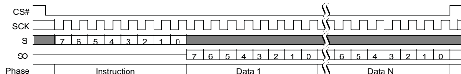
Figure 117. Password Read (PASSRD E7h) Command Sequence
