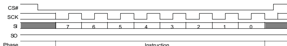
Figure 116. PPB Lock Bit Write (PLBWR A6h) Command Sequence
