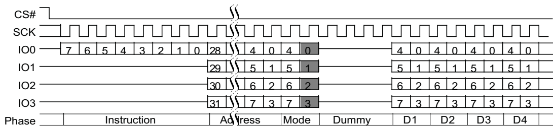
Figure 85. Continuous Quad I/O Read Command Sequence (4-Byte Address), LC=00b
