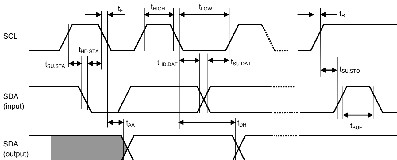
Figure 8 Bus Timing
