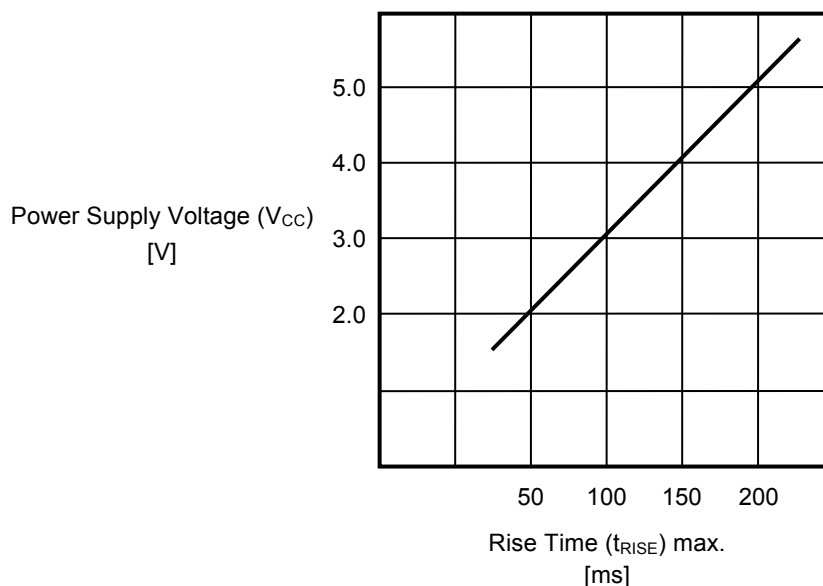
Figure 29 Rise Time of Power Supply Voltage
