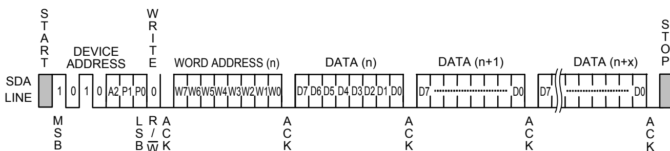
Figure 16 Page Write
