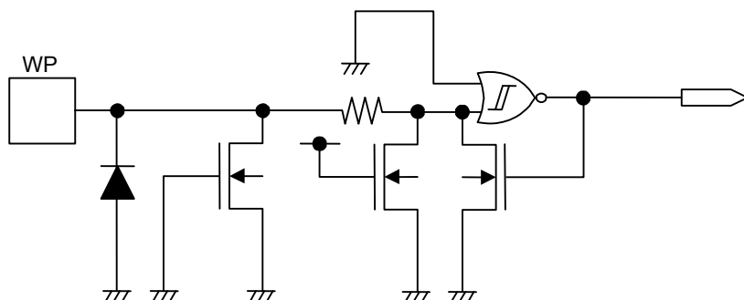
Figure 25 WP Pin
