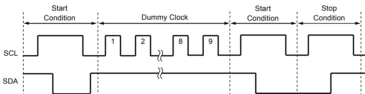
Figure 27 Resetting S-24C08C
