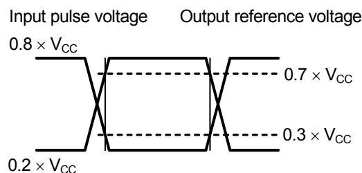
Figure 7 I / O Waveform during AC Measurement
