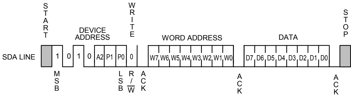
Figure 15 Byte Write
