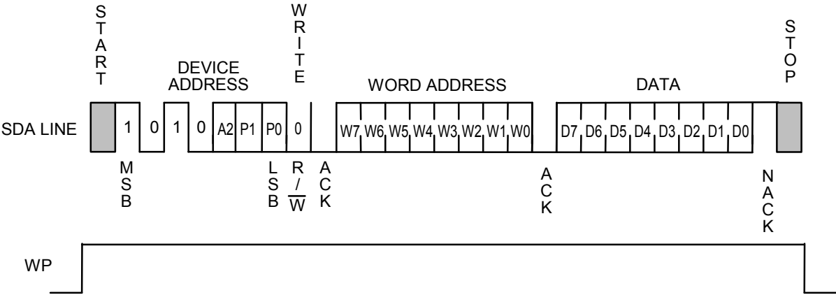
Figure 17 Write Protect
