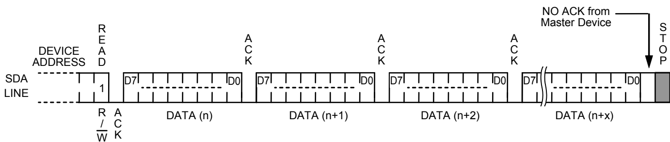
Figure 21 Sequential Read
