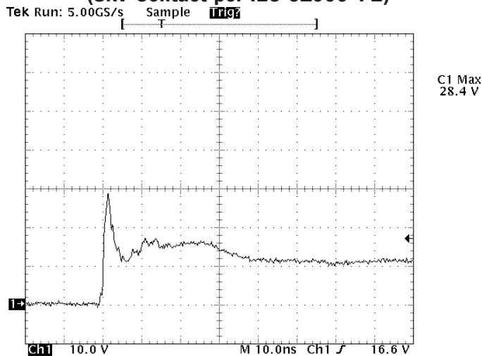
ESD Clamping
