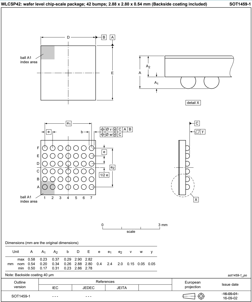
Figure 7. Package outline, WLCSP42, SOT1459-1
