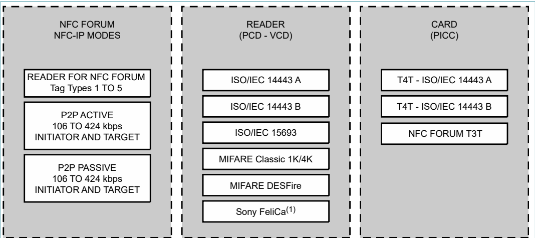
Figure 1. PN7150 transmission modes 1. According to ISO/IEC 18092 (Ecma 340) standard.
