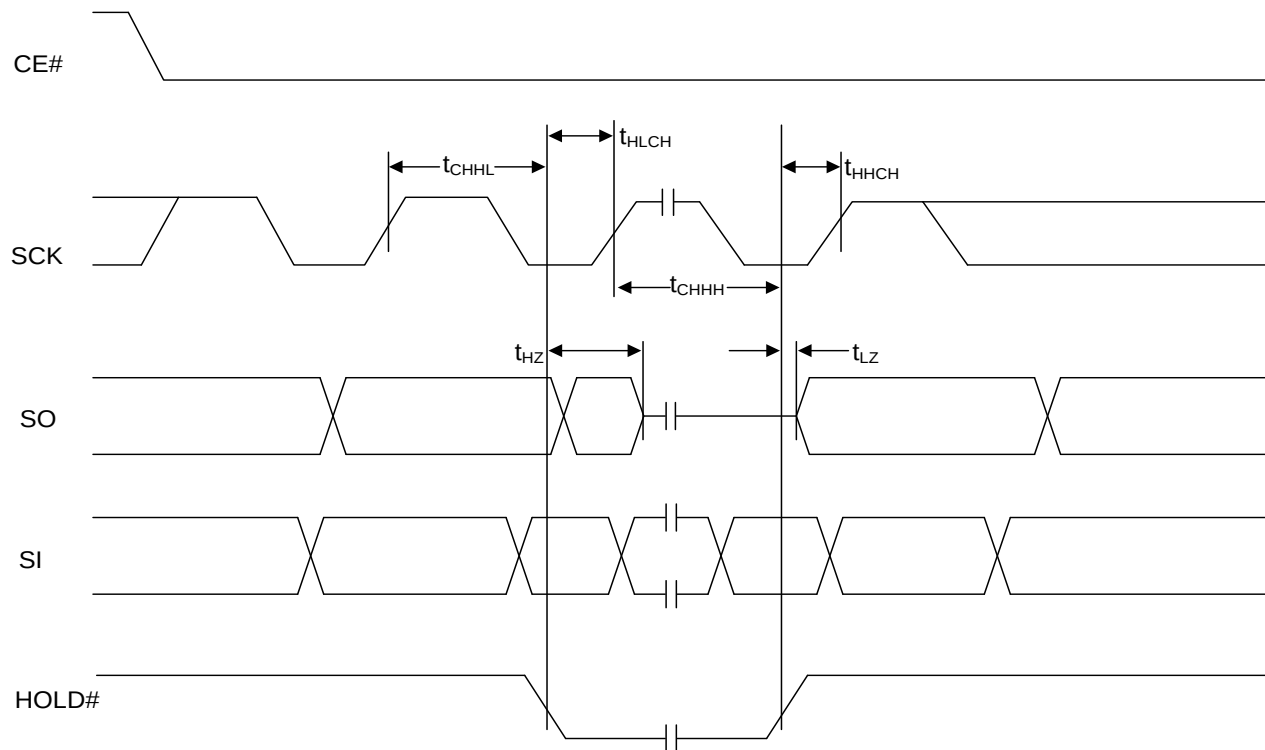
Figure 9.3 HOLD TIMING
