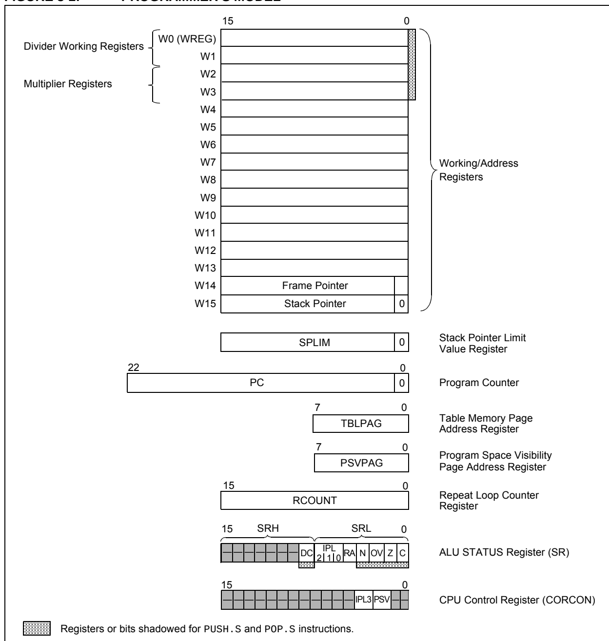
FIGURE 3-2: PROGRAMMER'S MODEL
