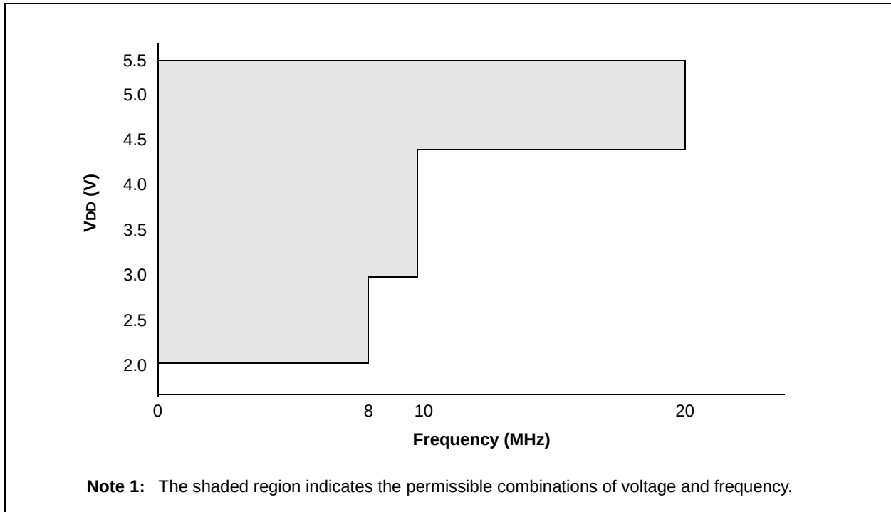
FIGURE 22-1: PIC16F753 VOLTAGE-FREQUENCY GRAPH, -40°C ≤ TA ≤ +125°C
