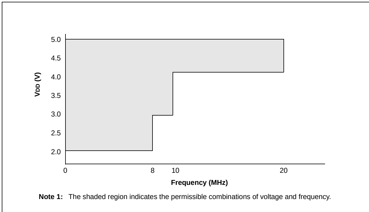
FIGURE 22-2: PIC16HV753 VOLTAGE-FREQUENCY GRAPH, -40°C ≤ TA ≤ +125°C
