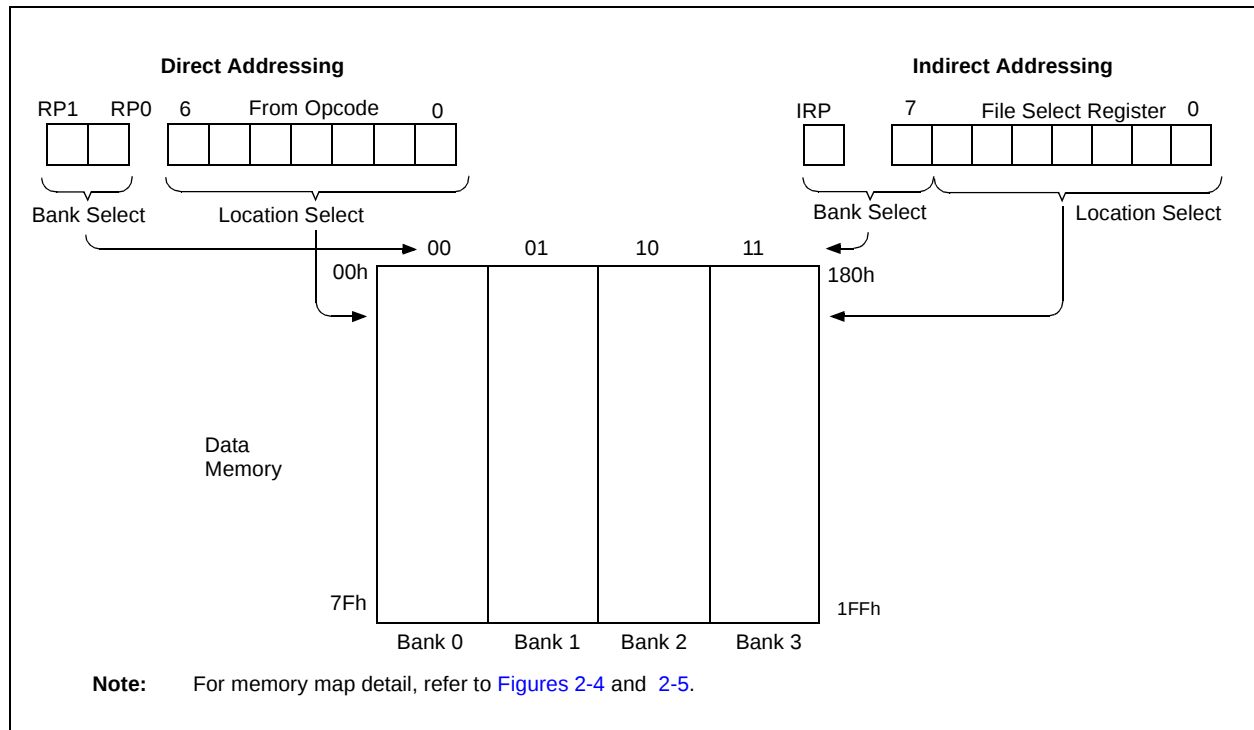
FIGURE 2-8: DIRECT/INDIRECT ADDRESSING
