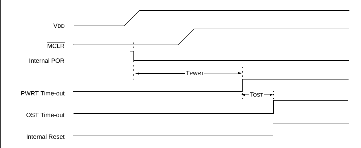
FIGURE 3-4: TIME-OUT SEQUENCE ON POWER-UP (DELAYED MCLR): CASE 1
