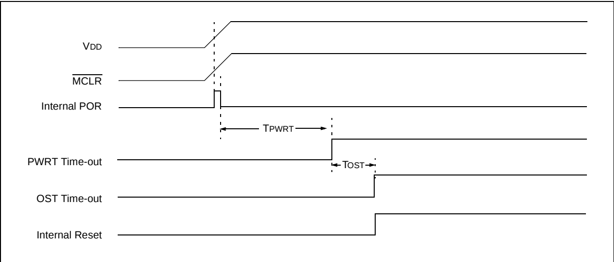
FIGURE 3-6: TIME-OUT SEQUENCE ON POWER-UP (MCLR WITH VDD): CASE 3
