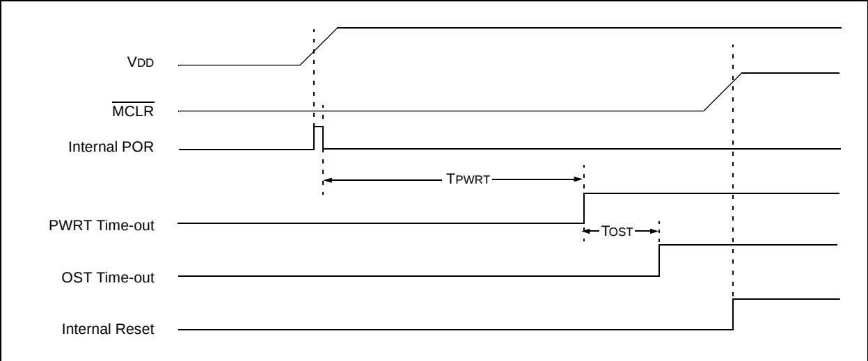
FIGURE 3-5: TIME-OUT SEQUENCE ON POWER-UP (DELAYED MCLR): CASE 2
