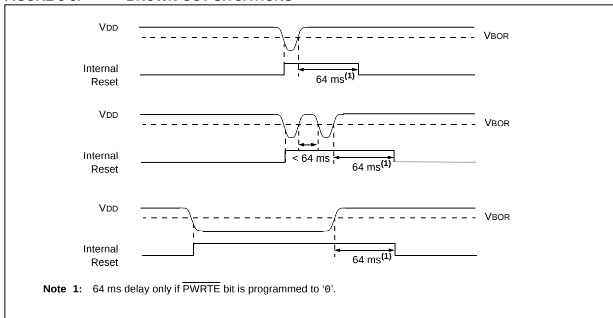
FIGURE 3-3: BROWN-OUT SITUATIONS
