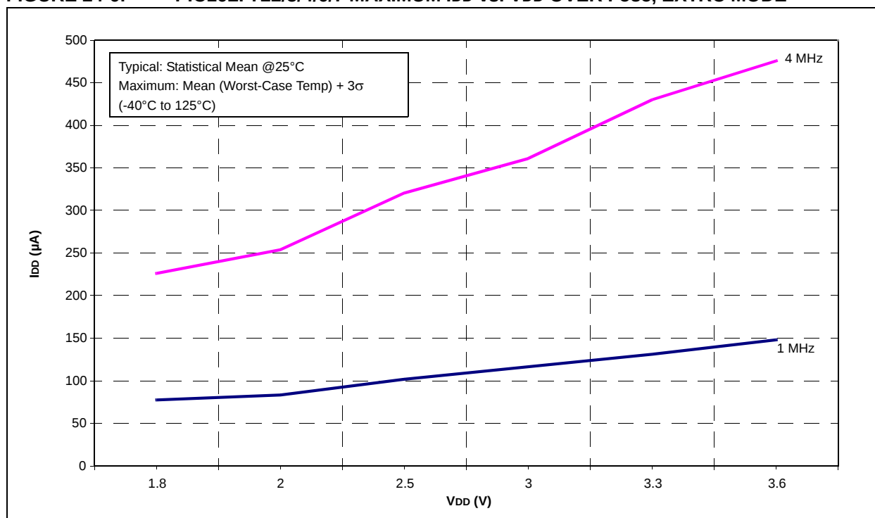
FIGURE 24-6: PIC16LF722/3/4/6/7 MAXIMUM I_{DD} vs. V_{DD} OVER F_{OSC} , EXTRC MODE
