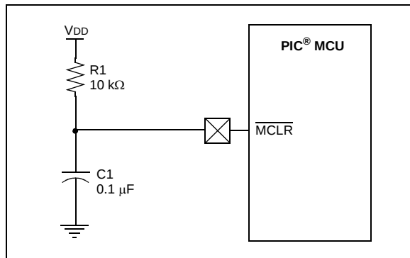
FIGURE 3-2: RECOMMENDED MCLR CIRCUIT
