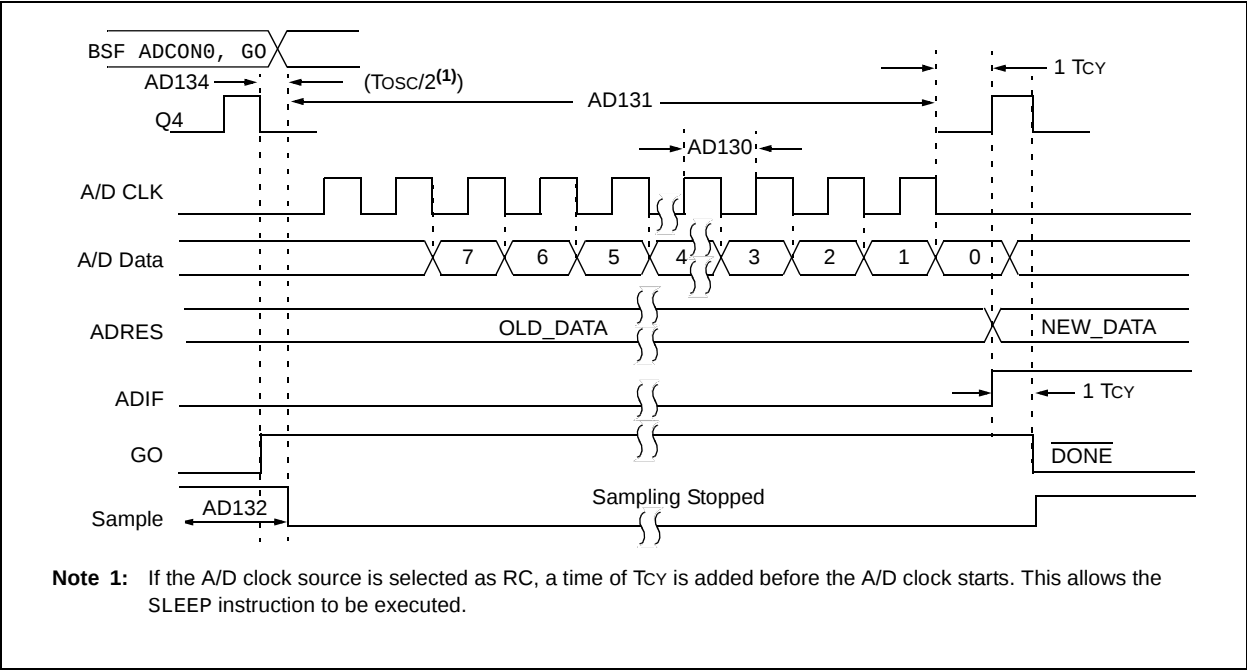
FIGURE 23-12: PIC16F722/3/4/6/7 A/D CONVERSION TIMING (NORMAL MODE)
