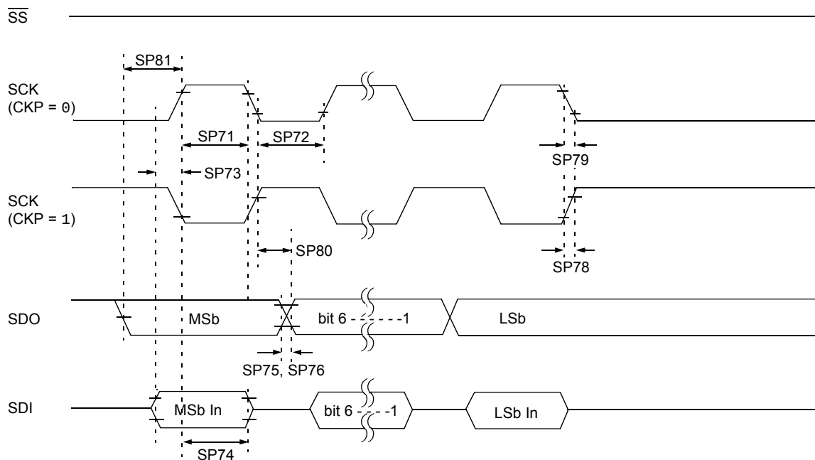
FIGURE 28-15: SPI MASTER MODE TIMING (CKE = 1, SMP = 1)
