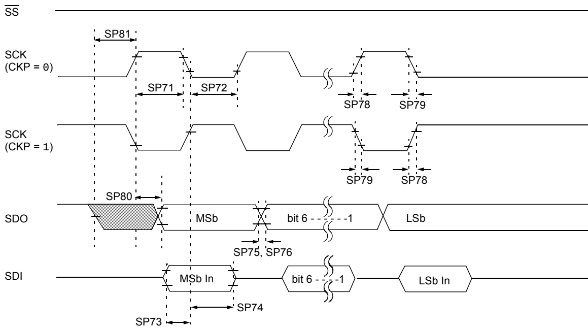
FIGURE 28-14: SPI MASTER MODE TIMING (CKE = 0, SMP = 0)
