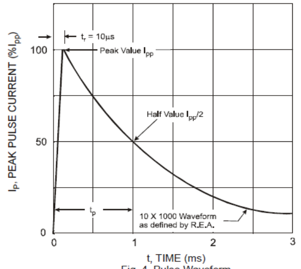
Fig. 4 Pulse Waveform
