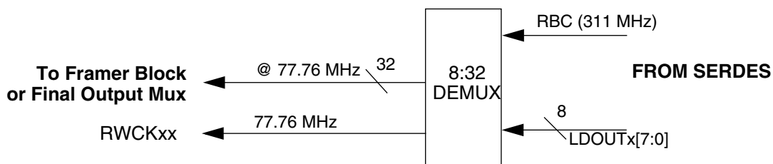
Figure 9. 8:32 DEMUX Block
