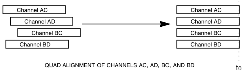
Figure 21. Quad Channel Alignment of SERDES Blocks A and B – ORSO42G5
