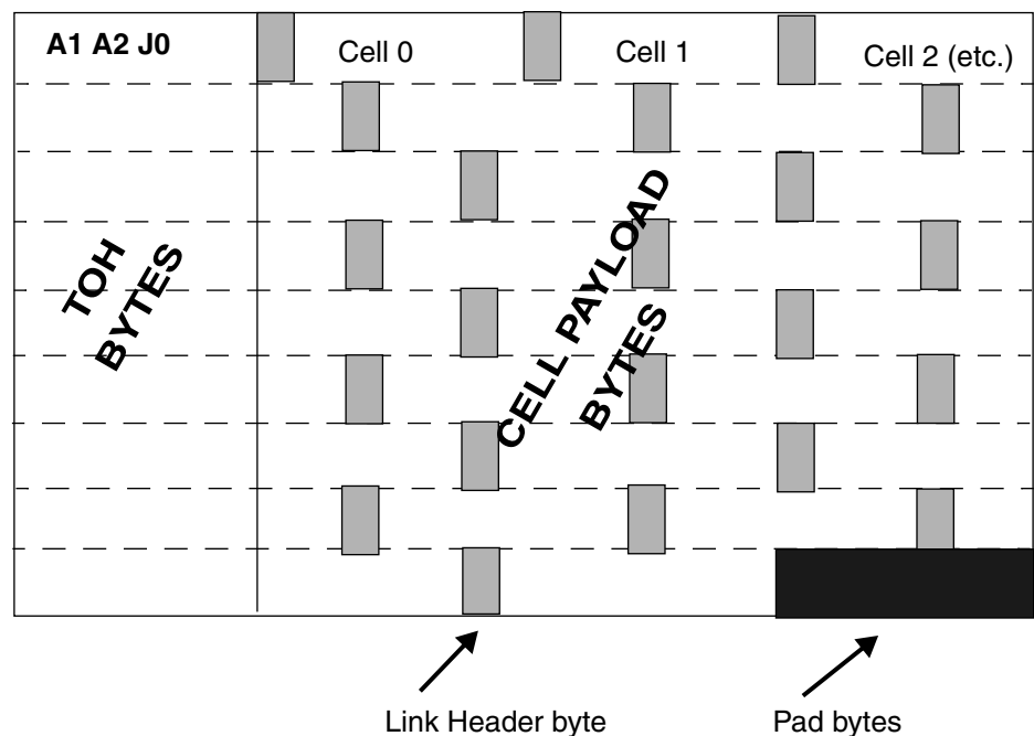
Figure 36. Cell Mapping in SONET Frame
