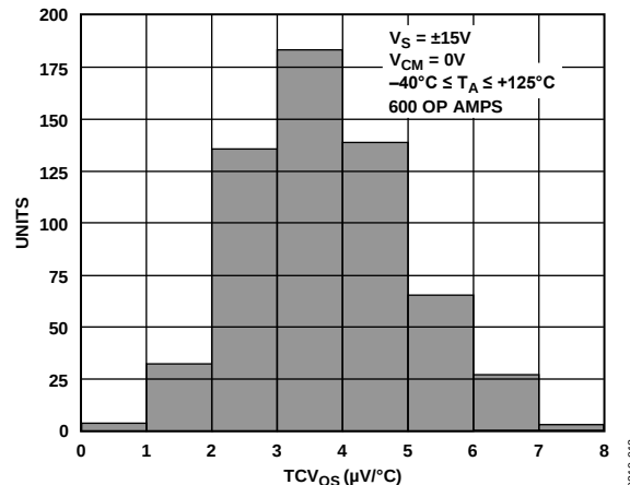
Figure 12. OP492 Temperature Drift ( TCV_{OS} ) Distribution @ \pm 15 V
