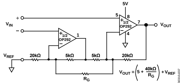
Figure 37. Single-Supply Instrumentation Amplifier
