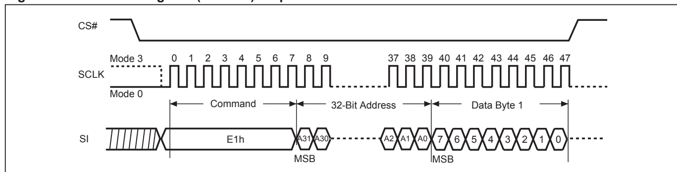
Figure 74. Write DPB Register (WRDPB) Sequence
