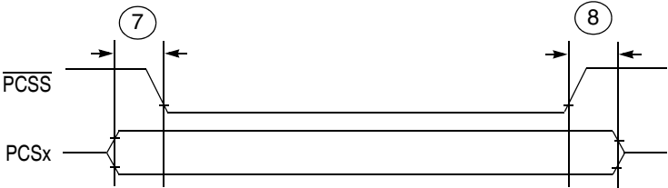
Figure 26. DSPI PCS Strobe ( \overline{\text{PCSS}} ) Timing
