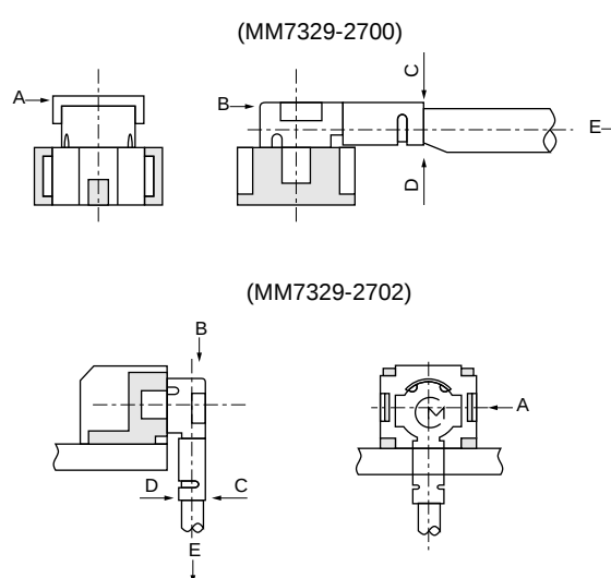
Figure 1. Mechanical Stress after Engagement
