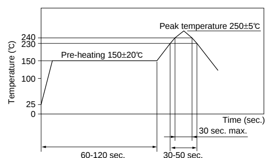
Reflow Soldering Standard Conditions
