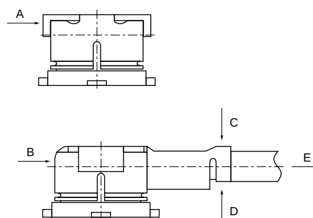
Figure 1. Mechanical Stress after Engagement
