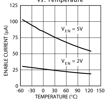
MIC29201/2 Shutdown Current vs. Temperature
