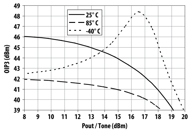
Figure 24. Over Temperature OIP3 vs Pout at 900 MHz
