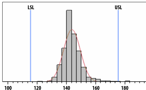
Figure 2. I_{dd} at V_{dd} = 5 V, LSL = 115 mA, Nominal = 146 mA, USL = 175 mA
