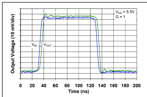
FIGURE 2-37: Non-inverting Small Signal Step Response.
