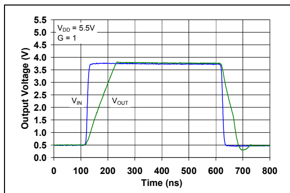
FIGURE 2-38: Non-inverting Large Signal Step Response.
