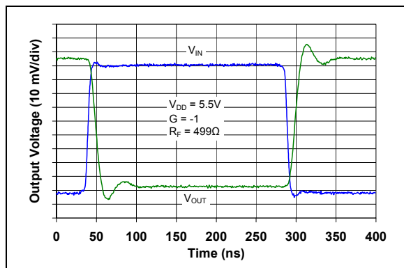
FIGURE 2-39: Inverting Small Signal Step Response.
