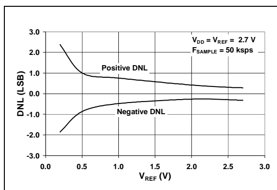
FIGURE 2-12: Differential Nonlinearity (DNL) vs. V_{REF} ( V_{DD} = 2.7\text{V} ).
