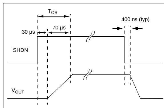
FIGURE 4-5: Shutdown Input Timing Diagram.
