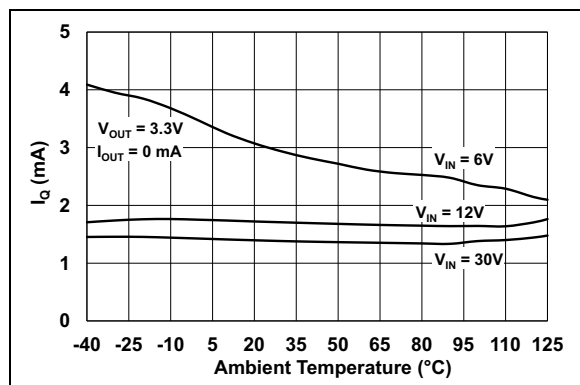
FIGURE 2-7: Input Quiescent Current vs. Temperature.
