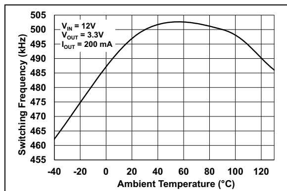
FIGURE 2-8: Switching Frequency vs. Temperature; V_{OUT} = 3.3V .
