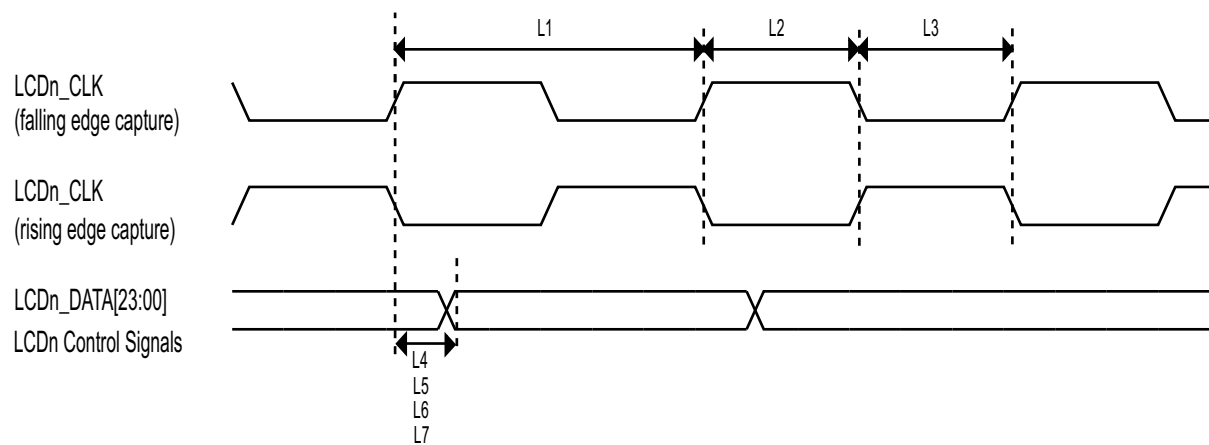
Figure 50. LCD Timing
