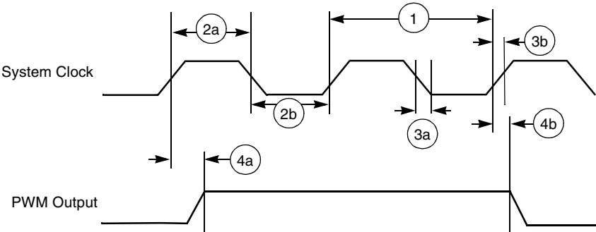
Figure 46. PWM Timing
