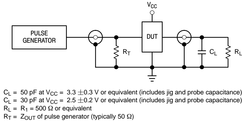
Figure 4. Test Circuit
