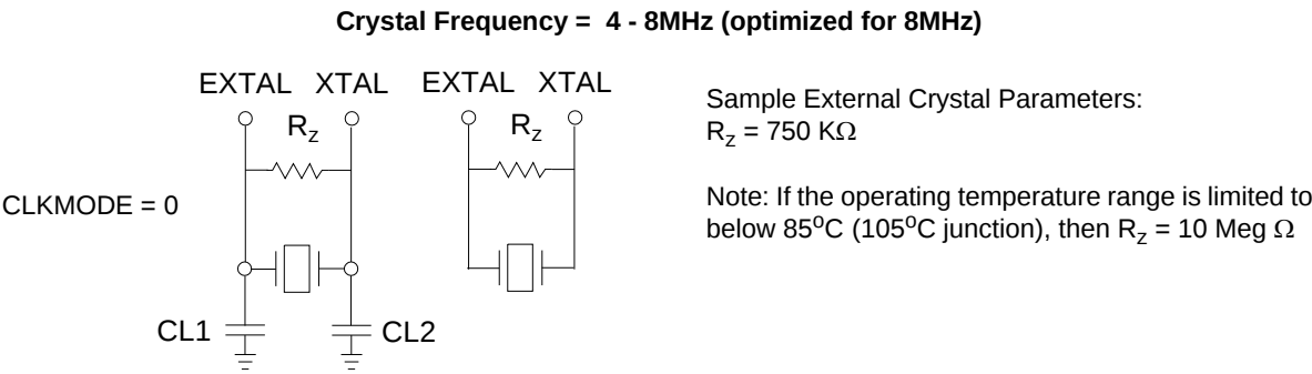
Figure 3-2 Connecting to a Crystal Oscillator
