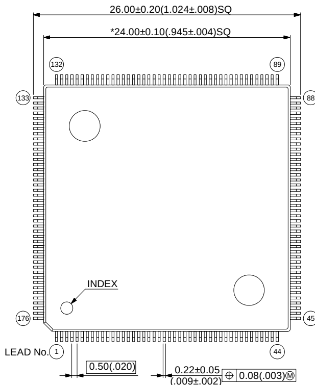
176-pin plastic LQFP (FPT-176P-M07)
