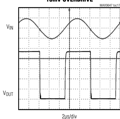
100kHz RESPONSE 10mV OVERDRIVE
