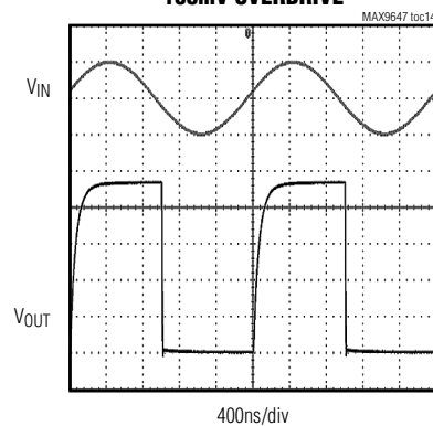
500kHz RESPONSE 100mV OVERDRIVE
