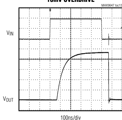
PROPAGATION DELAY 10mV OVERDRIVE
